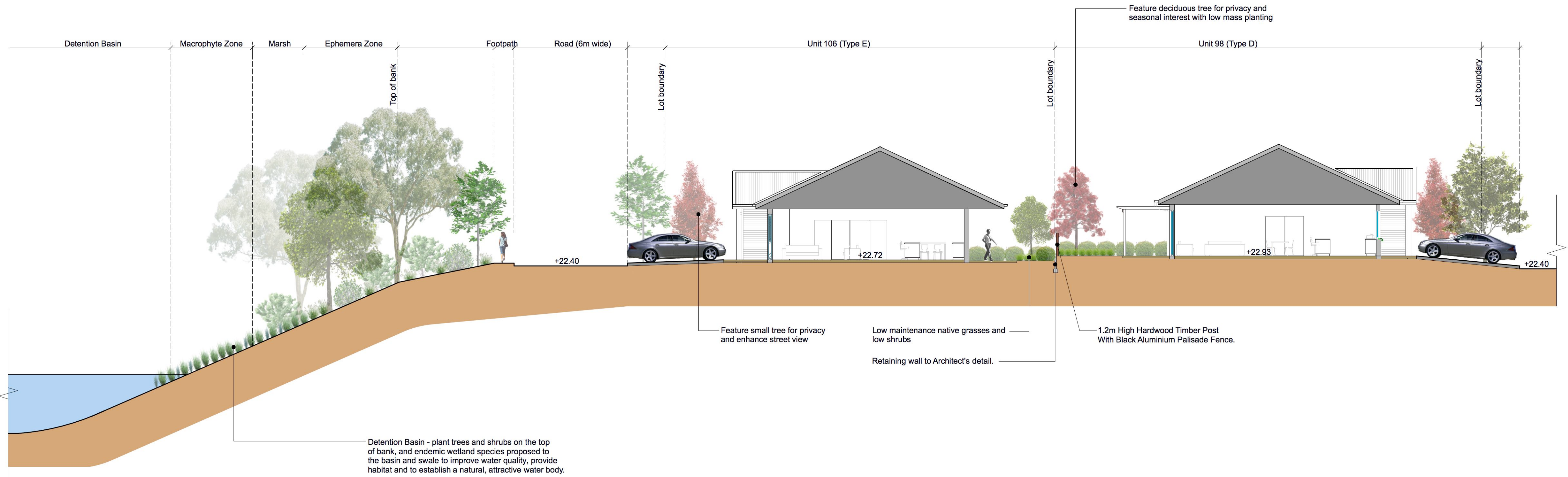
1.CROSS SECTION 1: 100 @ A1
